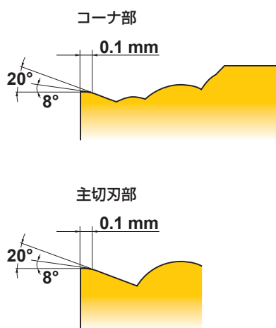
CNMG120408-FPH
